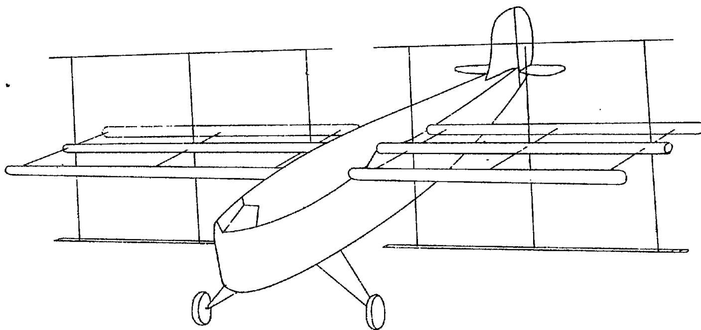
Figure 1.-The cyclogiro
