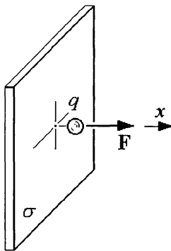
Fig. 10.11 A point charge q moves along the x axis under the action of a charged plate carrying a surface charge \sigma . This system can be used as a primitive clock.
