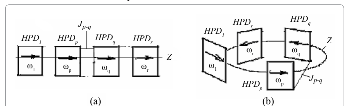
Figure 9: Two versions of sequence of HPDs ( HPD_1, \dots, HPD_p, \dots, HPD_q, \dots, HPD_r ), with respective precession frequencies \omega_1, \dots, \omega_p, \dots, \omega_q, \dots, \omega_r , aligned with the tangent to Z: (a) the linear configuration, (b) the circle configuration. J_{p-q} is spin supercurrent.
