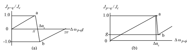
Figure 8: Normalized spin supercurrent J_{p-q}/J_c as a function of \Delta\omega_{p-q}t ( t is time, \Delta\omega_{p-q} is the difference in precession frequencies of HPD_p and HPD_q ). The line a-b corresponds to the phase slippage by the value of 2\pi . For (a) \Delta\alpha_c = \pi , for (b) \Delta\alpha_c > 2\pi ; g = 1 - b_1 2\pi .
