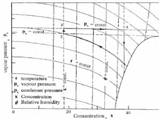
Figure 3. Absorption-regeneration cycle [1].
