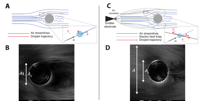
Fig. 1. Trajectories of fog droplets around a cylinder with and without the application of corona discharge. (A and B) Schematic of air streamlines and droplet trajectories and photograph of droplet trajectories in the absence of an electric field. The inset shows the velocities of the wind \vec{w} and the particle \vec{u} and the drag force acting on the droplet. The bright ring is the edge of the cylinder. (C and D) Schematic of air streamlines, electric field lines, and droplet trajectories and photograph under corona discharge. Droplets closely follow the electric field lines in this case. The inset shows the additional electric force acting on a droplet. The cylinders in (B) and (D) have a diameter of 1.88 mm.
