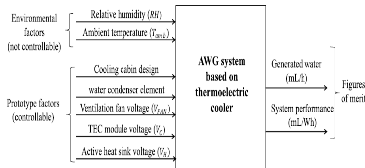
Fig.4 - Factors affecting the AWG system & the figure of merits
