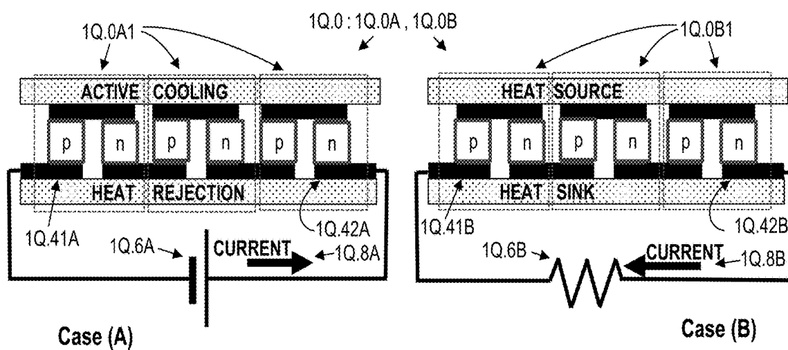
Prior Art Fig. 1q
