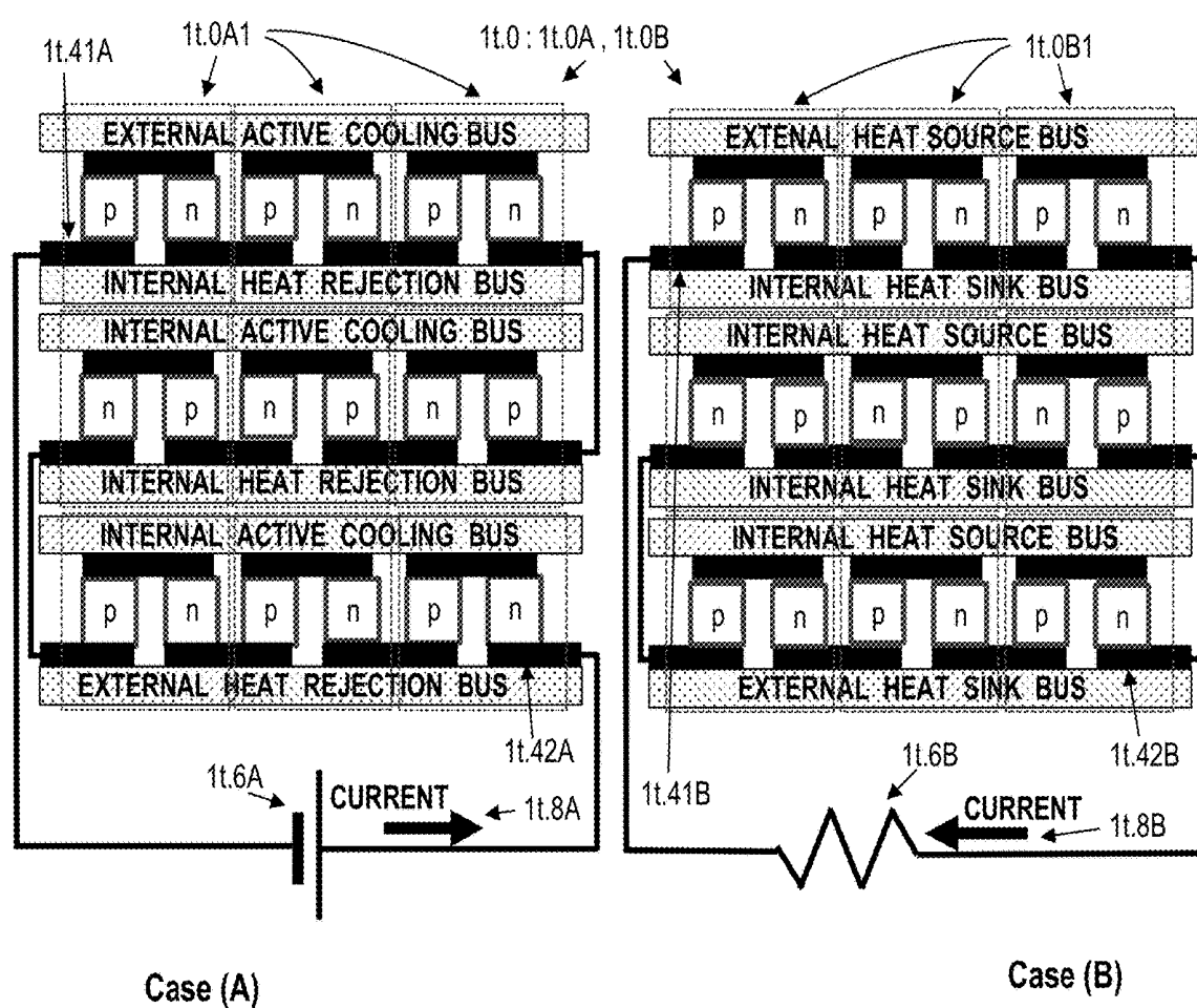
Prior Art Fig. 1t
