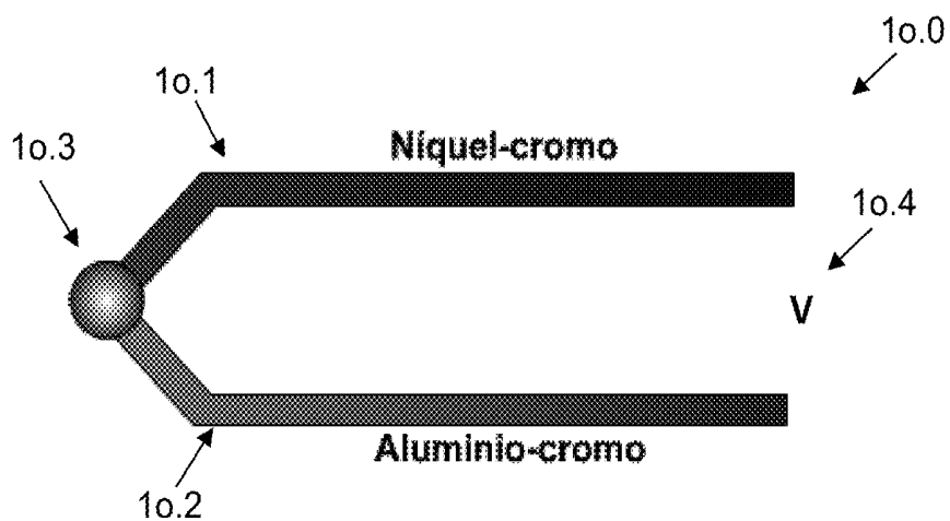
Prior Art Fig. 1o
