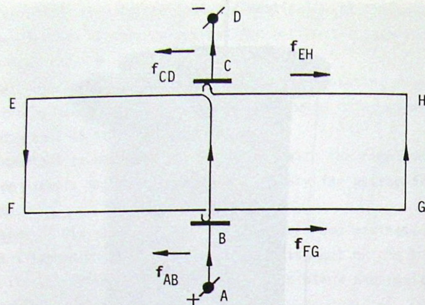
Fig. 70. Sigalov's second experiment.
