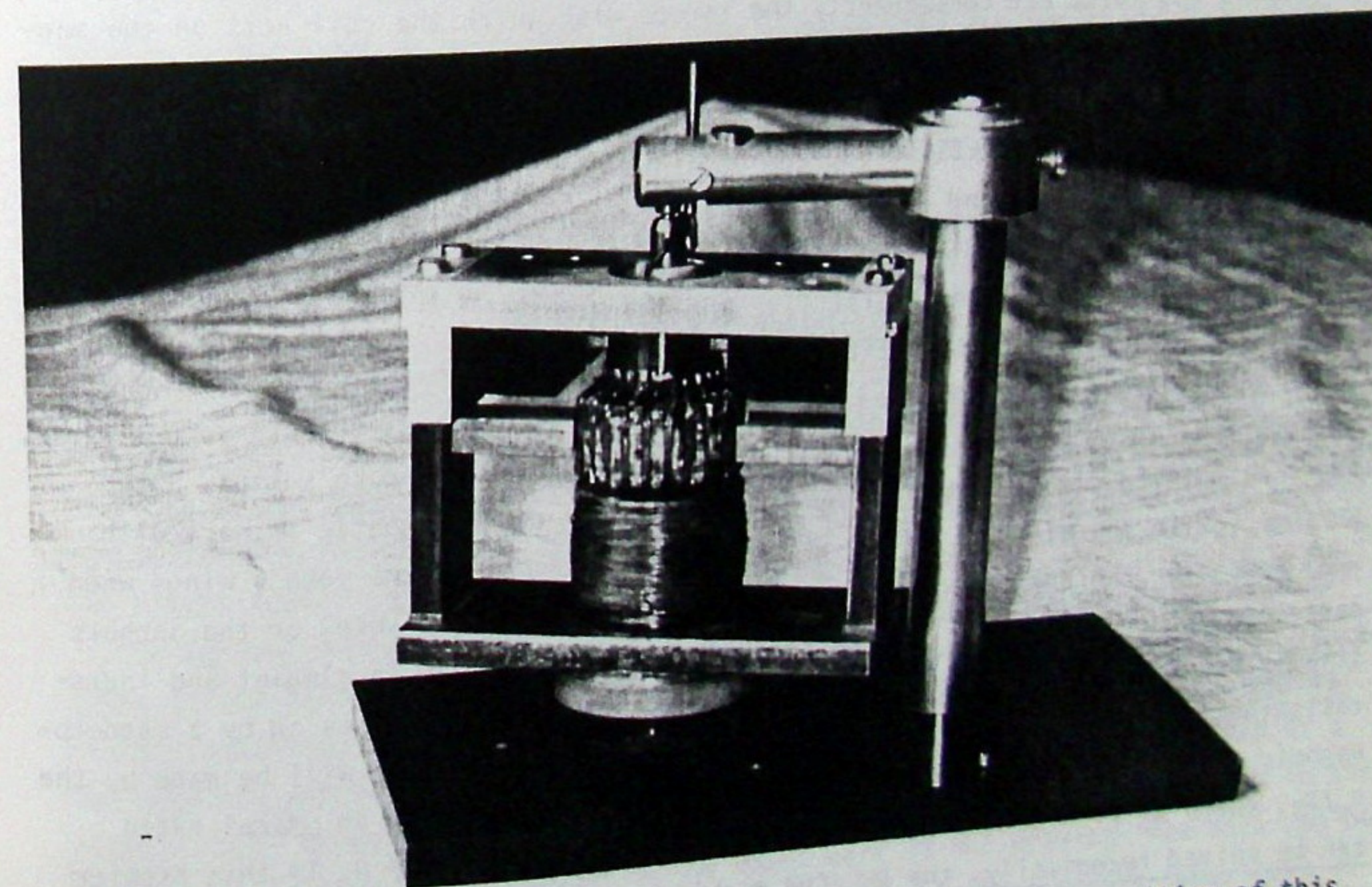
Fig. 32. Second variation of the effective BUL-CUB machine. The position of this machine corresponds to the position of Müller's machine in fig. 29.
