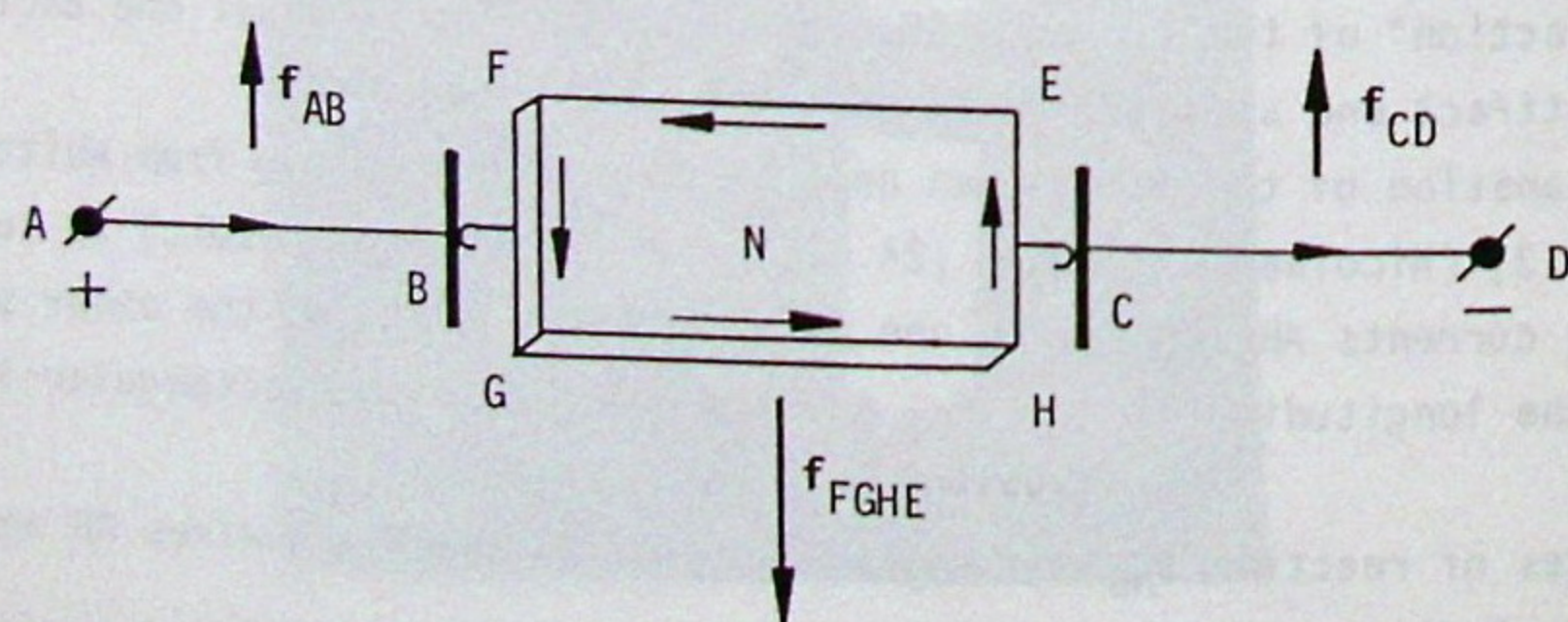
Fig. 71. Sigalov's third experiment.
