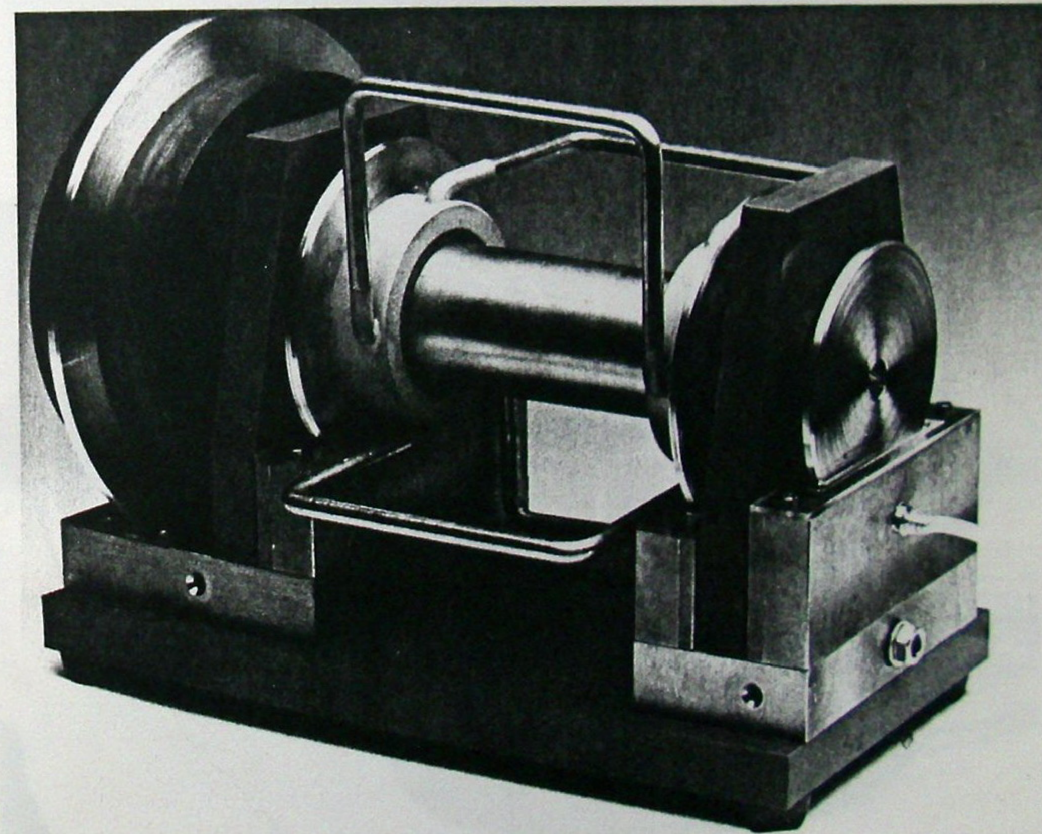
Fig. 64. Photograph of the RAF-machine.
