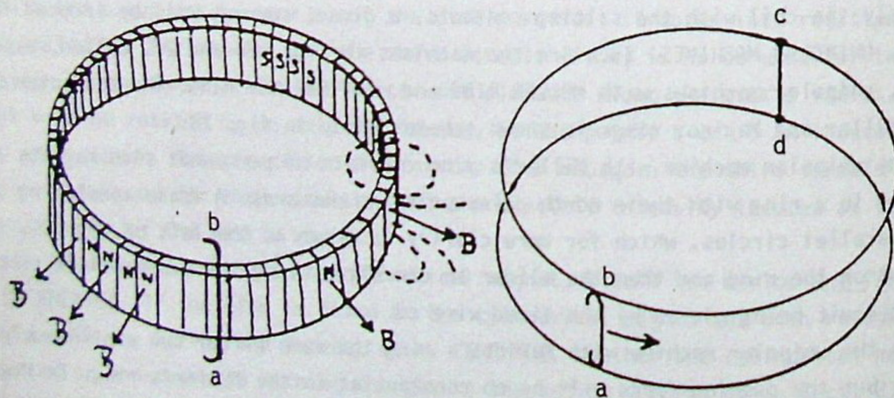
Fig. 26. Unipolar machine with Müller's ring.
