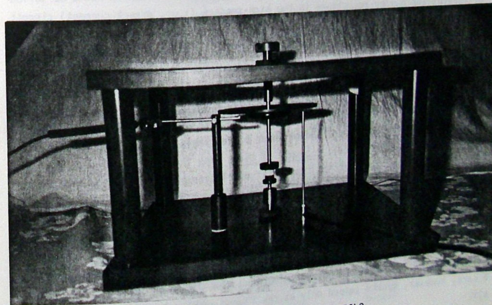
Fig. 84. Photograph of the S-motor MODRILO.
