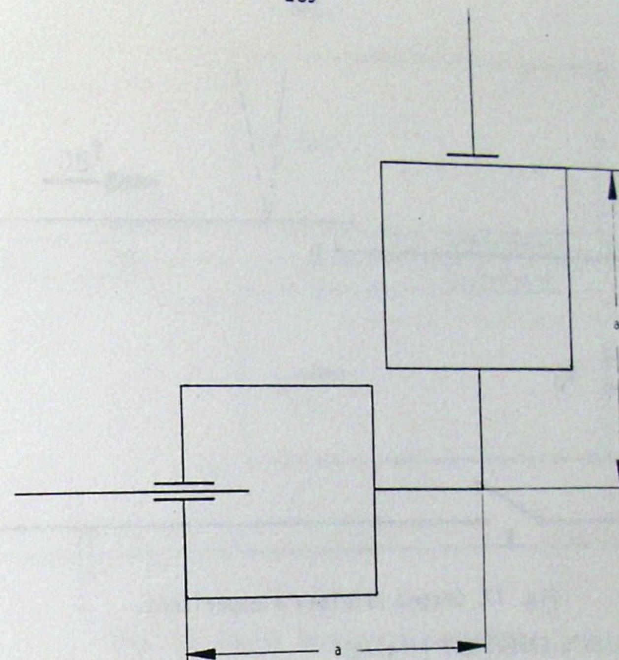
Fig. 76. Realization of the sliding contacts at the corners of Nicolaev's first experiment permitting exact calculation of the acting forces.
