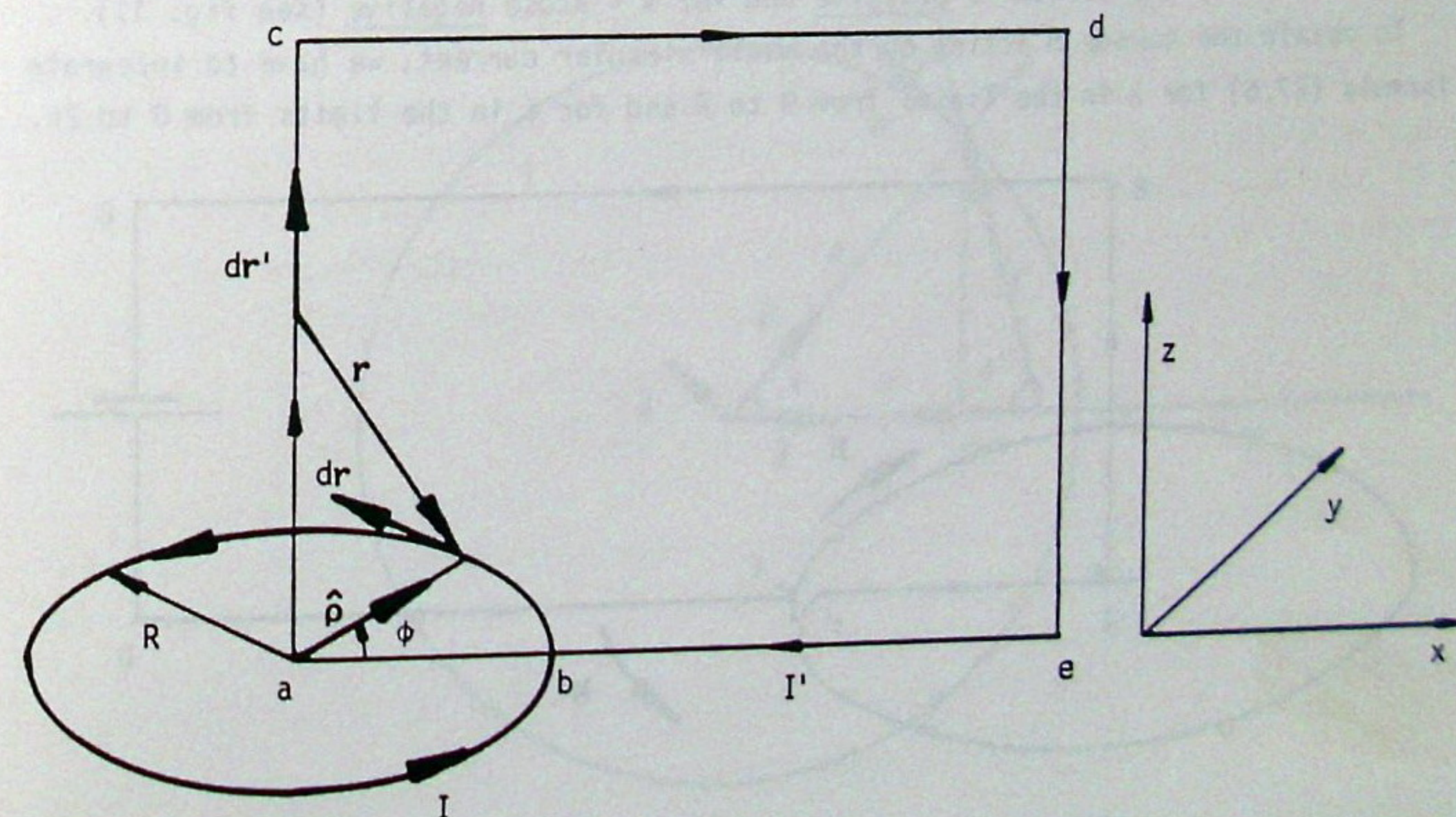
Fig. 9. Rectangular and circular circuits.
