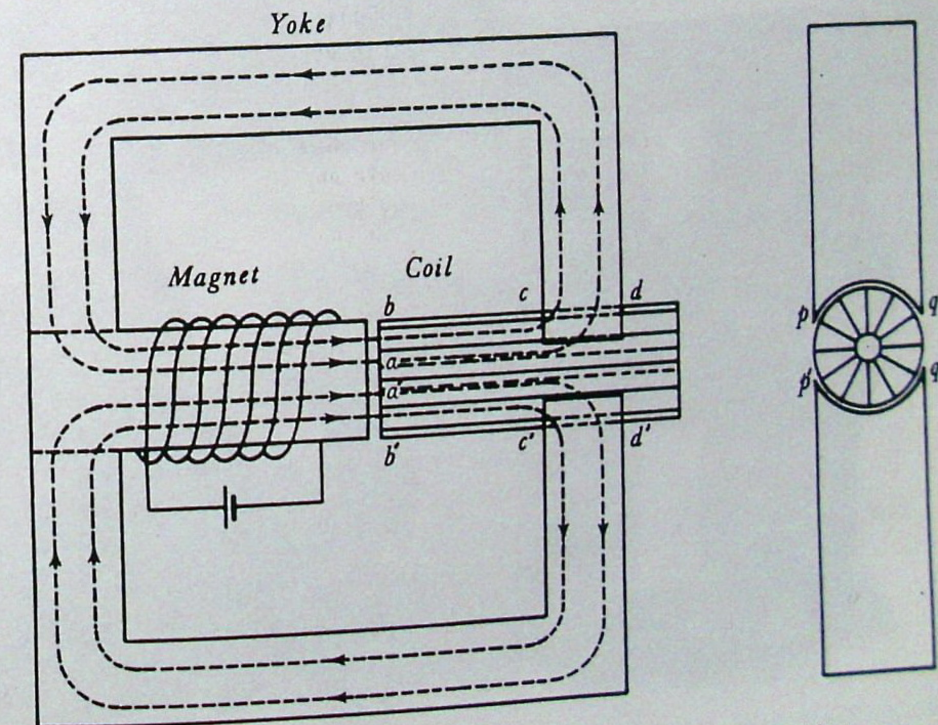
Fig. 30. Diagram of the one-and-a-half polar BUL-CUB machine.
