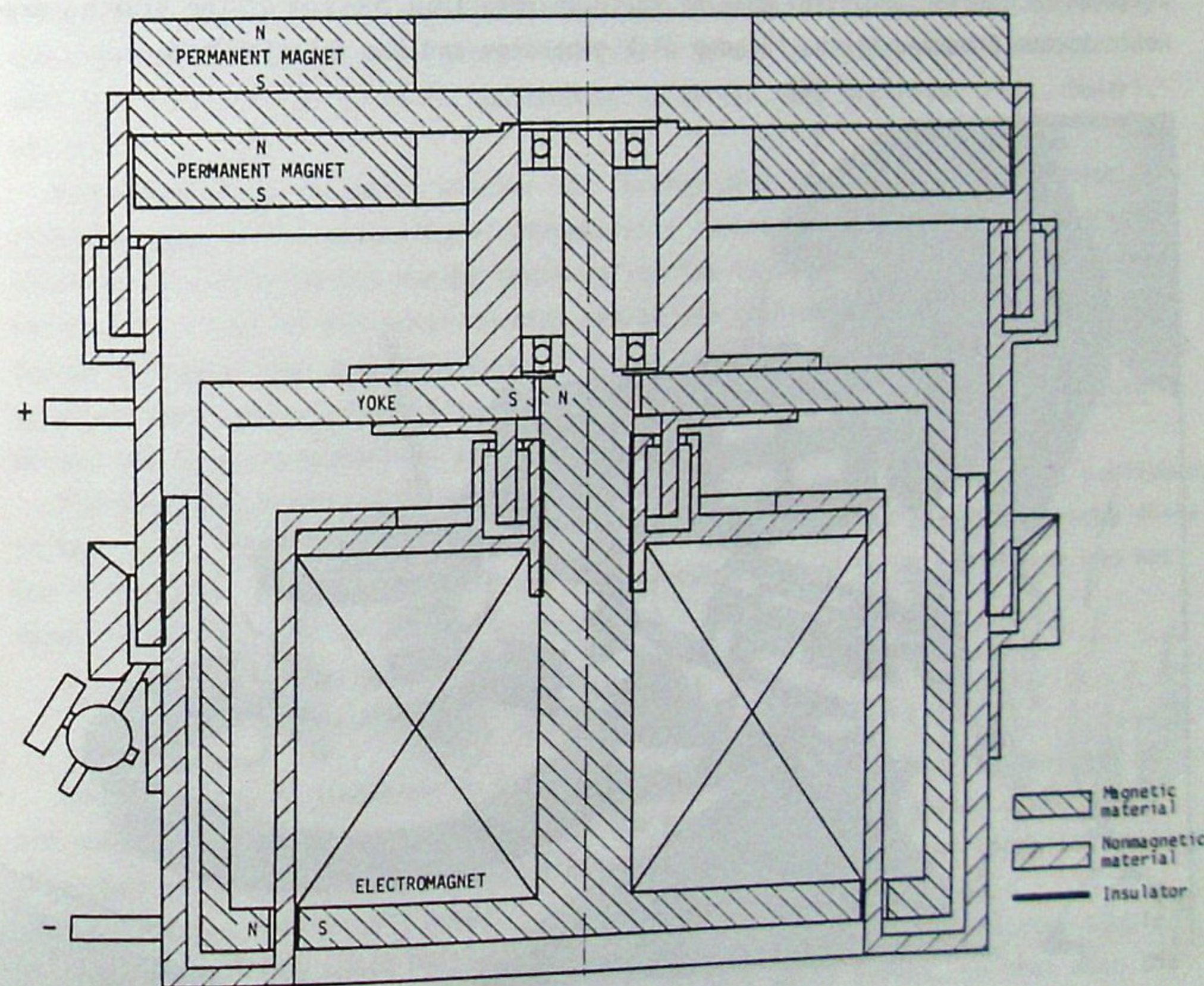
Fig. 38. Diagram of the open half polar machine ADAM.
