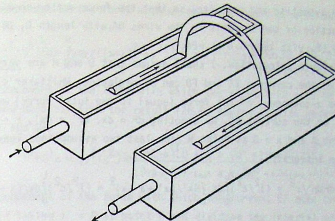
Fig. 7. The classical propulsive Ampere bridge.
