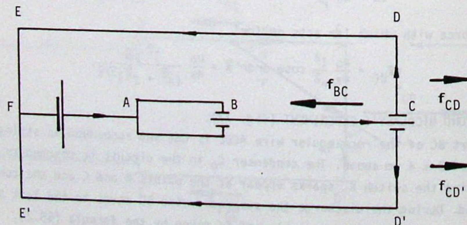
Fig. 78. Third Nicolaev's experiment.
