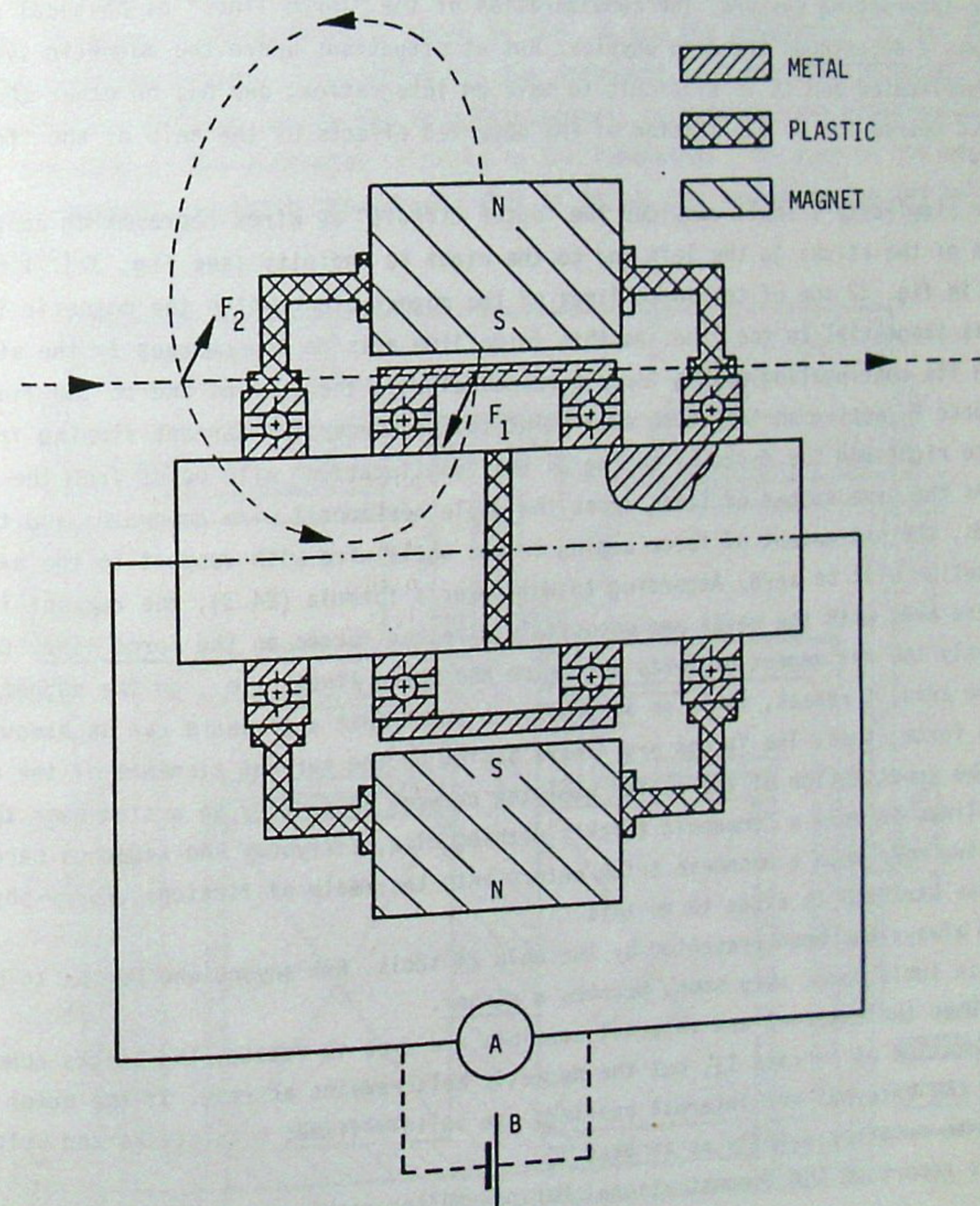
Fig. 37. Diagram of the demonstrational unipolar Marinov-Müller machine.
