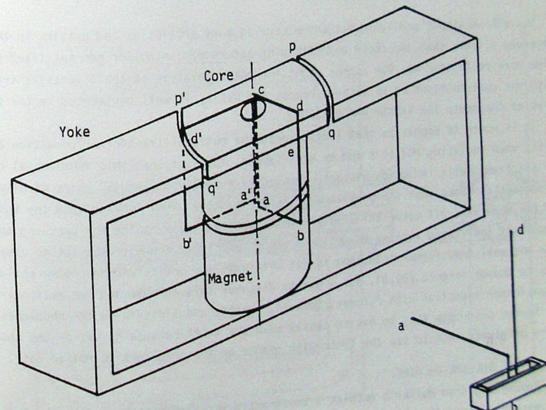
Fig. 29. Müller's one-and-a-half polar machine.
