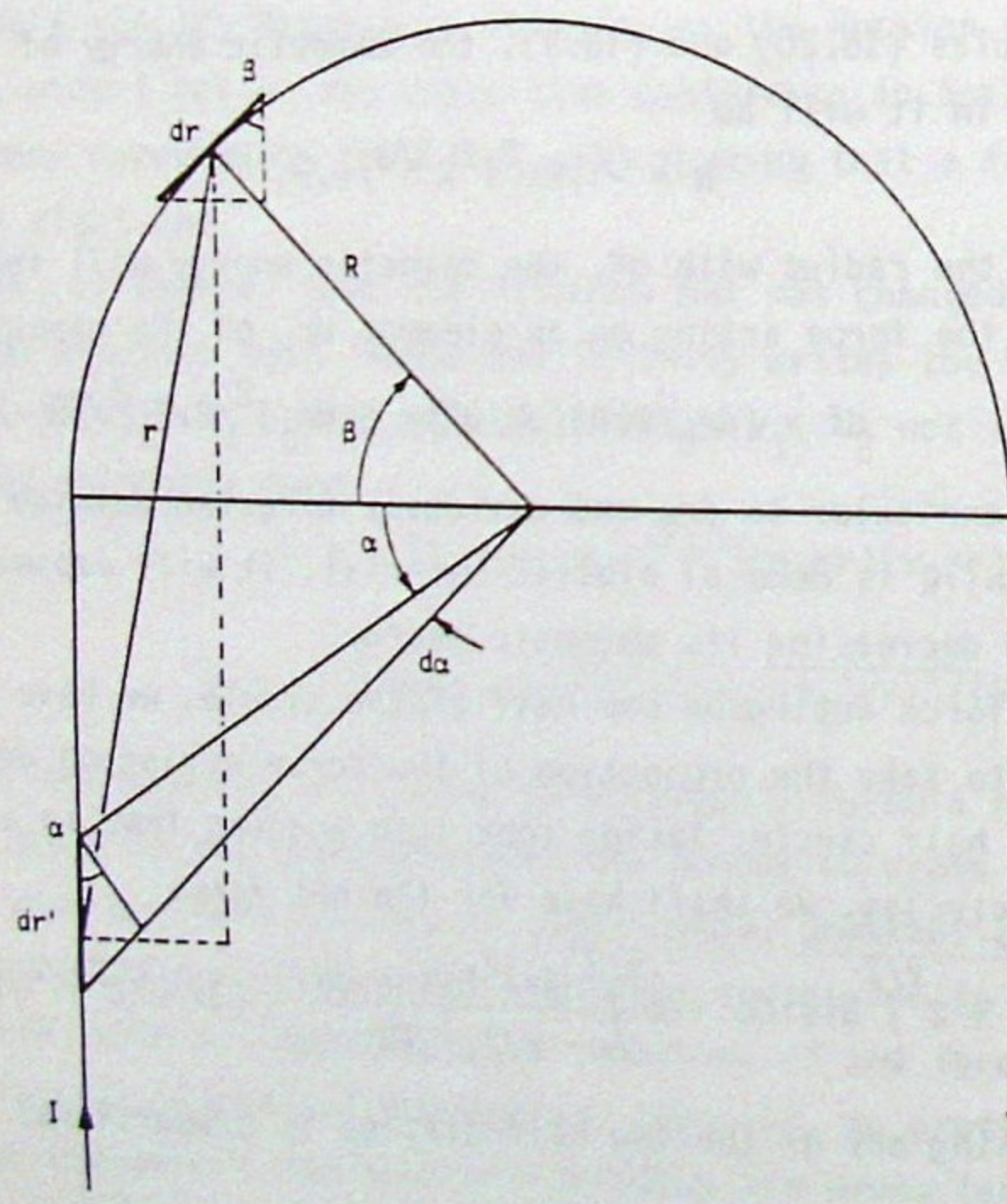
Fig. 6. Half-circular propulsive Ampere bridge.
