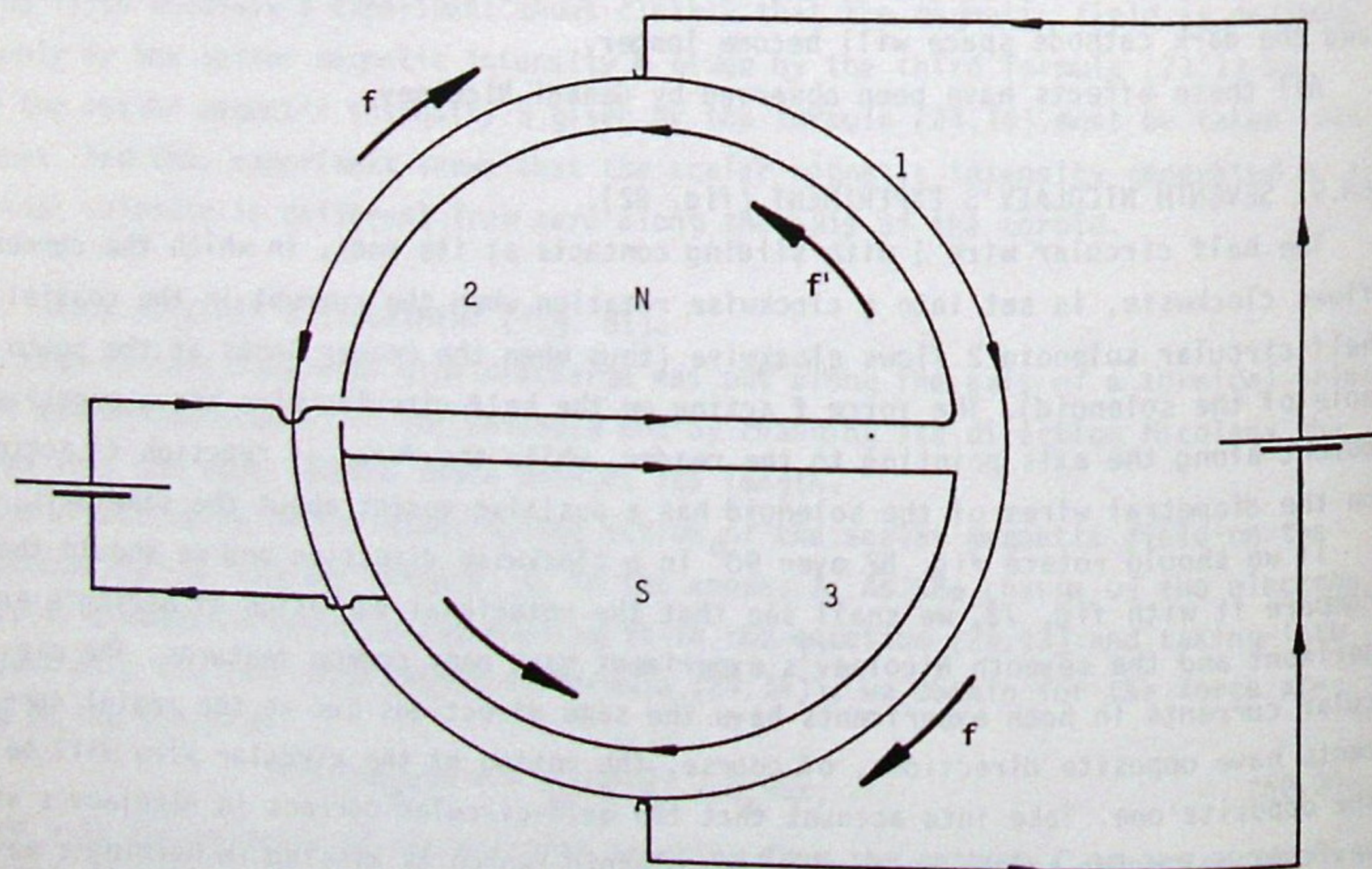
Fig. 83. Eighth Nicolaev's experiment.
