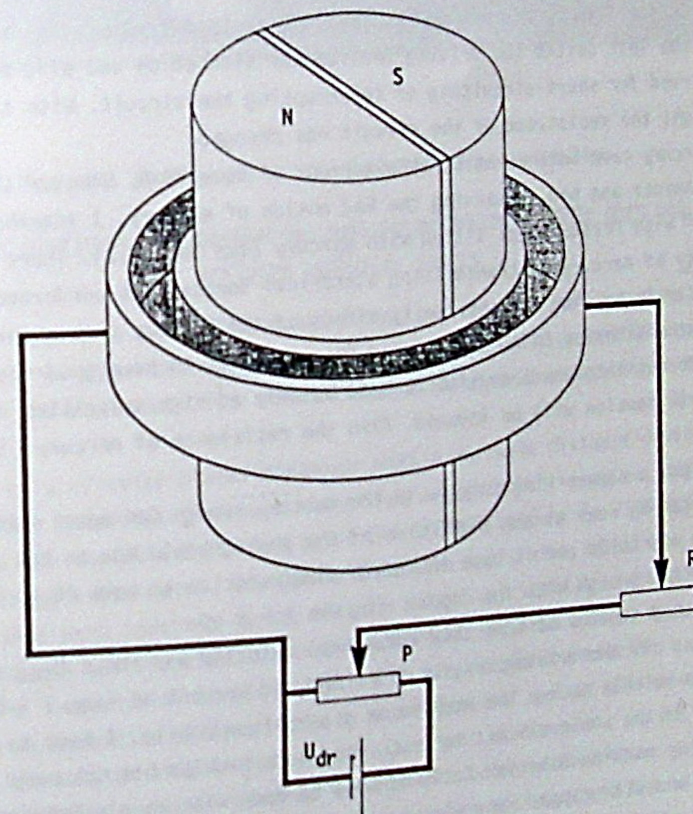
Fig. 87. The S-machine Siberian Coliu with liquid rotating ring.
