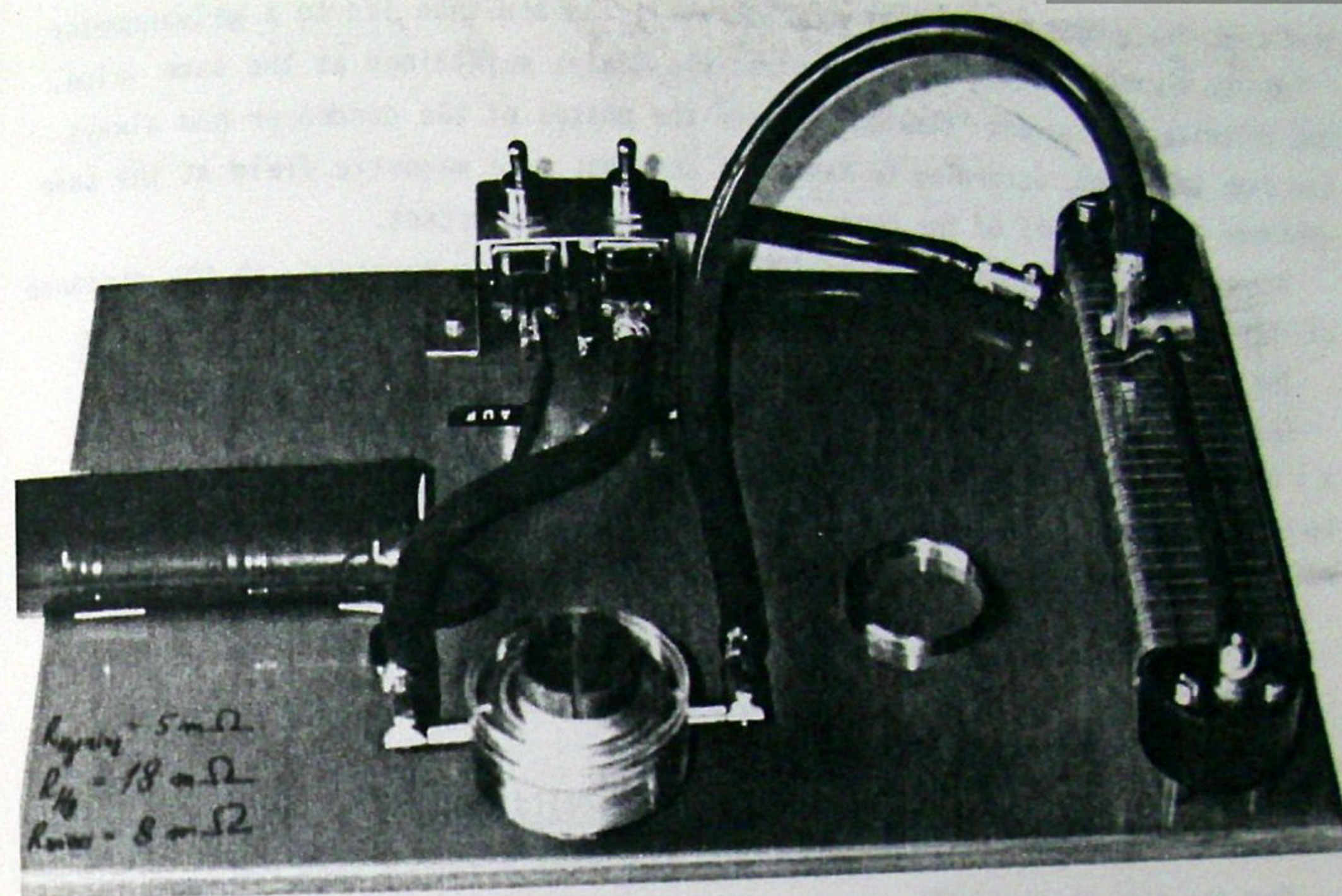
Fig. 88. Photograph of the S-machine Siberean Coliu.
