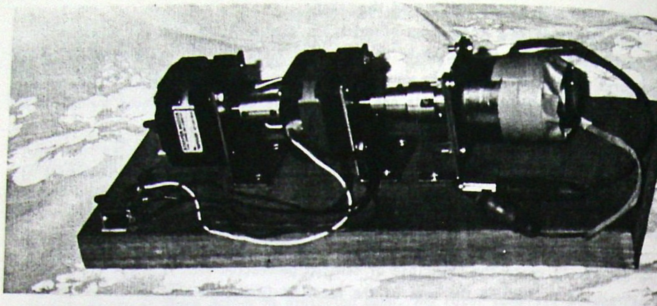
Fig. 50. Two mechanically coupled stepping motors (used as generators) driven by a common d.c. motor.
