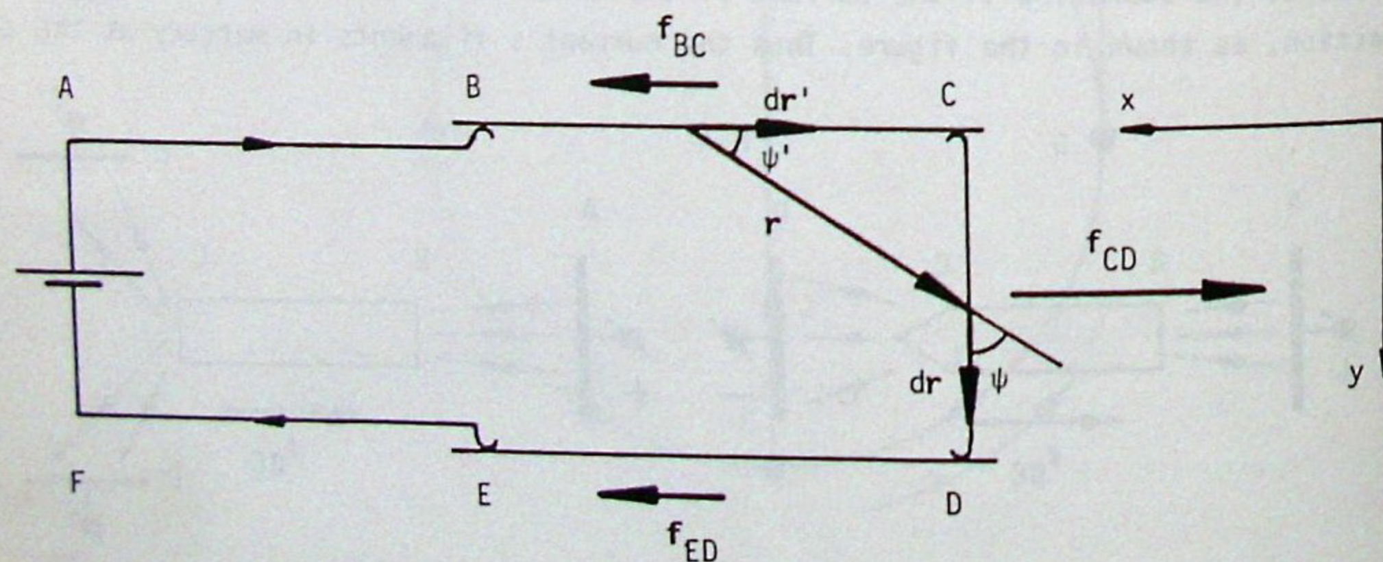
Fig. 75. First Nicolaev's experiment.
