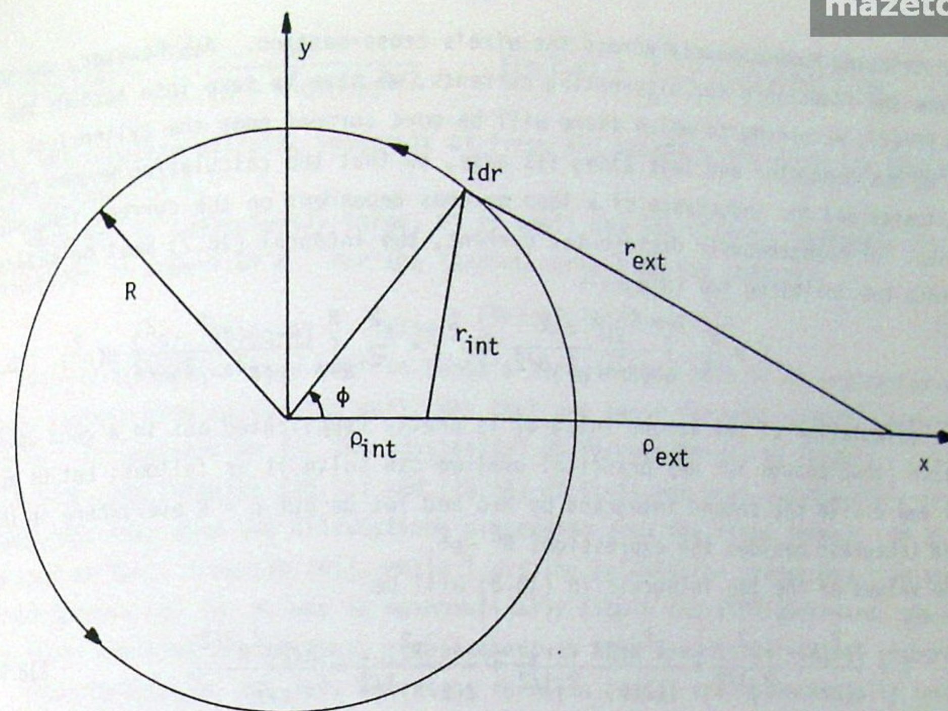
Fig. 2. Circular loop in which current flows.
