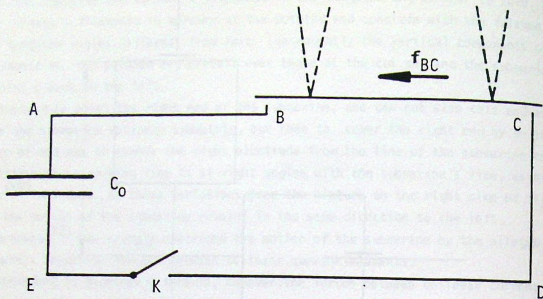
Fig. 77. Second Nicolaev's experiment.
