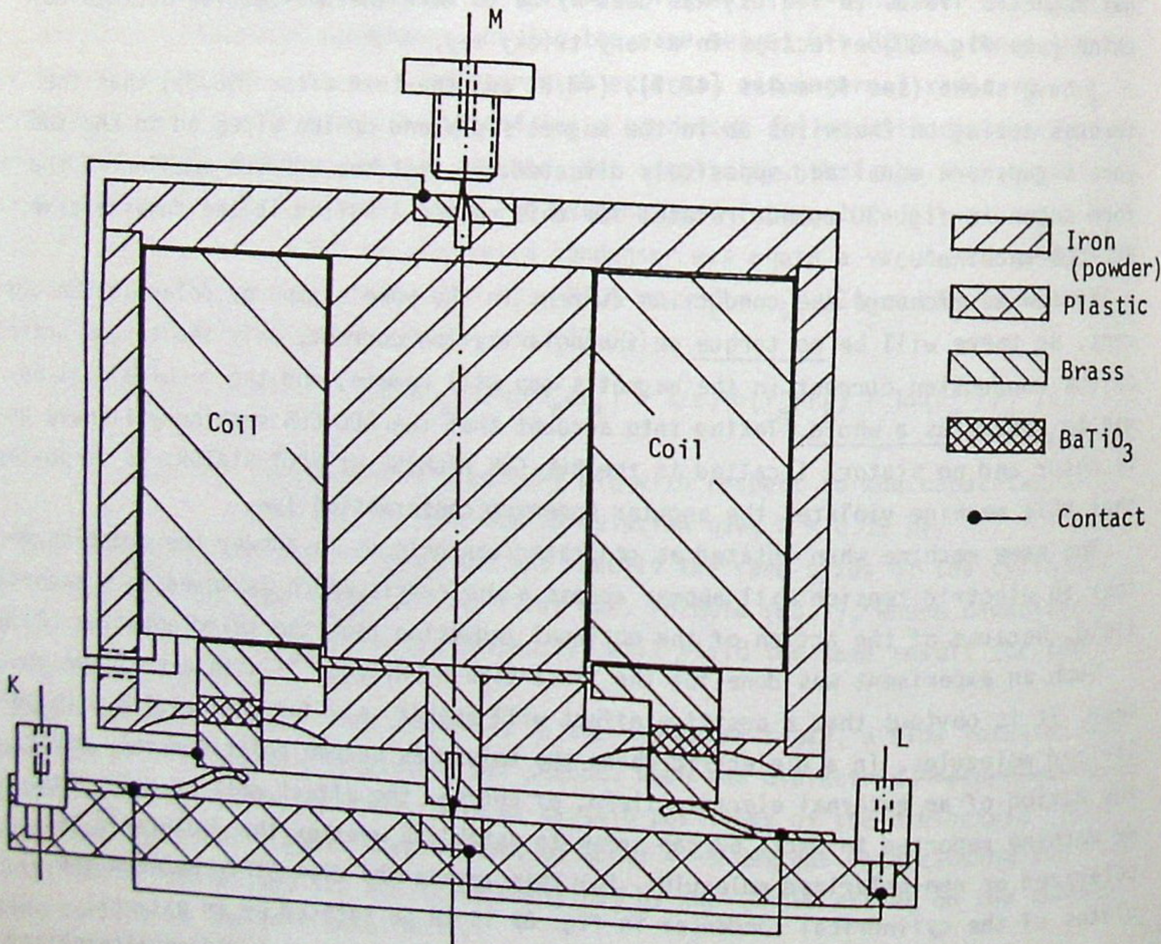
Fig. 92. Diagram of the BUL-CUB machine without stator.
