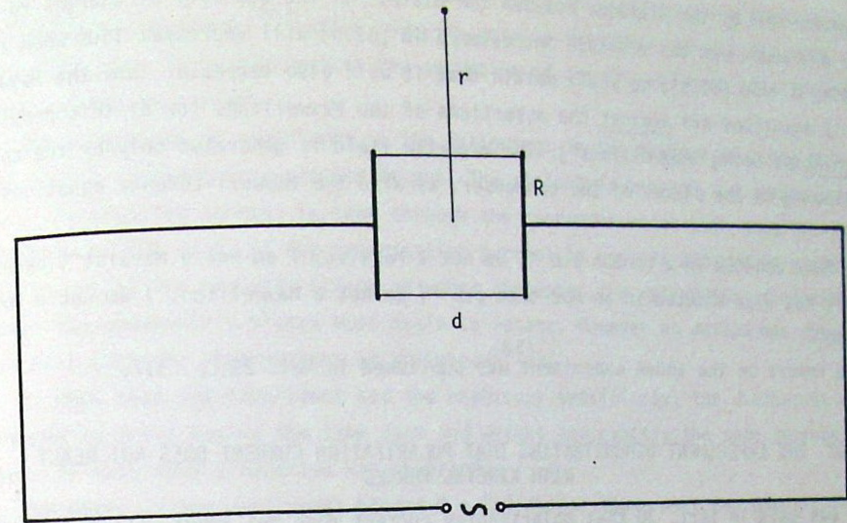
Fig. 89. Diagram of the experiment showing that polarization current does not act with potential magnetic forces on other currents.
