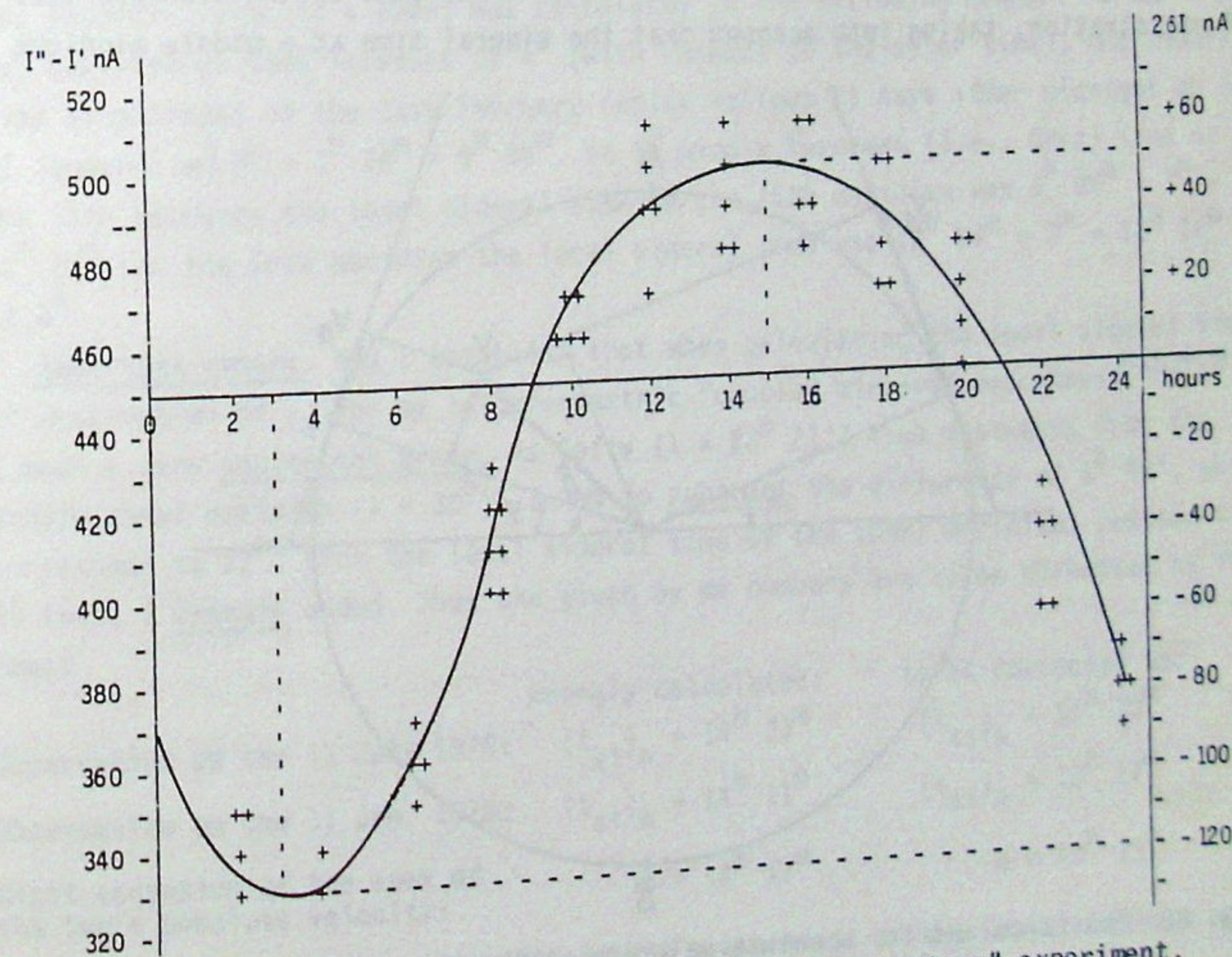
Fig. 19. Measurement of 2\delta I in the "coupled shutters" experiment.
