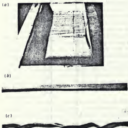
Figure 3. Buckling of thin rails (B): (a), inward deflection of aluminium rails; (b), steel rail before recoil experiment; (c), steel rail after recoil experiment.
