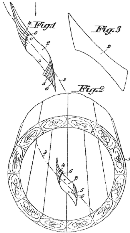
Drawing for patent 138296, guide vanes in wooden water pipe
