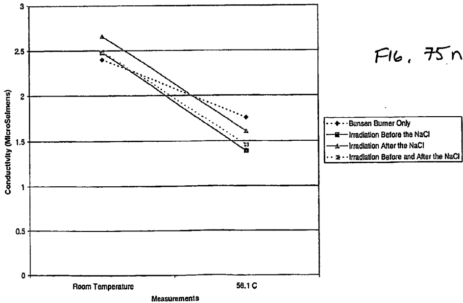
Conductivity - Averages of 4 Different Experimental Conditions
