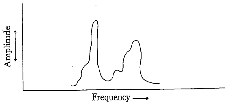
Spectral pattern at moderate temperature
