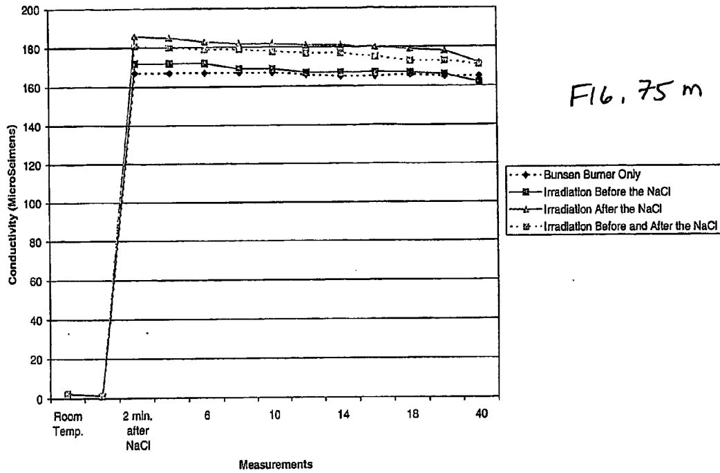
Conductivity - Averages of 4 Different Experimental Conditions
