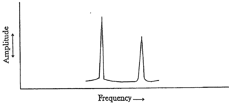
Separate and distinct spectral curves at low temperature
