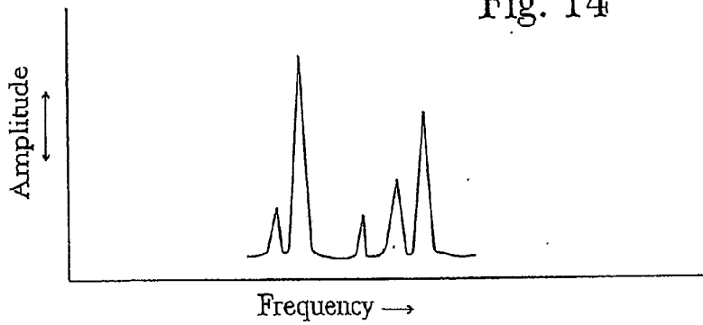
Spectral pattern at low temperature
