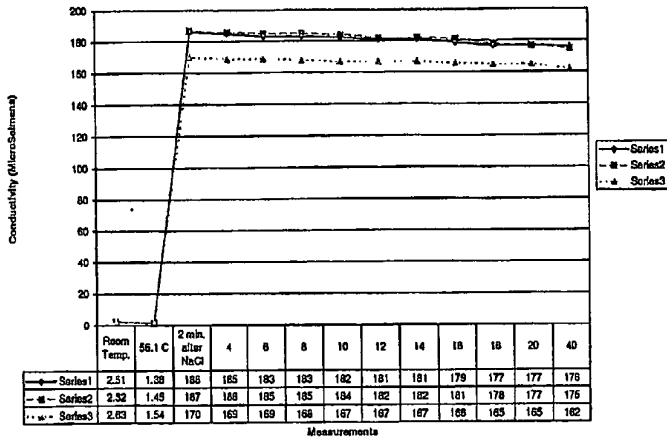
4. Conductivity - Sodium Irradiation Before and After the Salt imp
