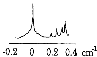
High resolution spectrum Fig. 31
