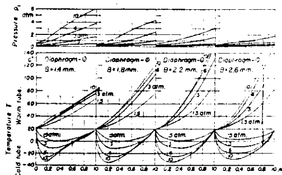
FIG. 2: Temperature of cold and hot gas stream and internal pressure in tube No. 1 as function of external pressure, size of diaphragm, and \mu . \mu = mass of cold/mass of total air. Constants: R=4.6 mm, D=1.1 mm, T_0=20^\circ\text{C} , p_a=1 atmos. Parameter: pressure p at the nozzle.
