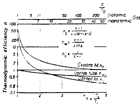
FIG. 5. Efficiency of 3 refrigerating machines for comparison.
