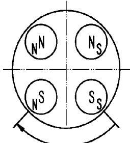
DEAD ZONE 180°
