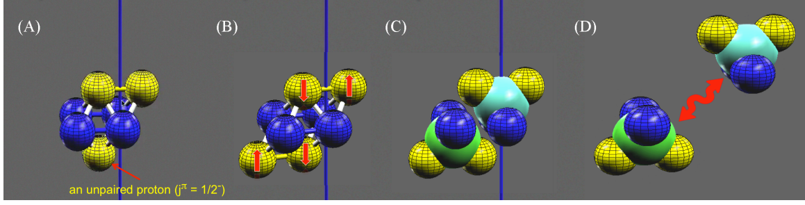
Figure 5: The lowest-lying excited-state of {}^7_3\text{Li}_4 (A) has a lattice structure to which an additional proton will produce a two-tetrahedron structure, giving {}^8_4\text{Be}_4 (B). The double alpha lattice structure (C) can then break into independent two alpha particles (D), which are released with 17 MeV of angular momentum, but without gamma radiation.
