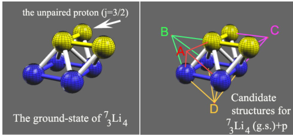
Figure 4: (Left) The ground-state of {}^7_3\text{Li}_4 . Among several dozen theoretical possibilities, the lattice locations of the last two paired-neutrons and the last unpaired-proton, as shown here, provide a J\pi value ( 3/2^- ) that is in agreement with experiment. A mirror-image isomeric state has the same properties. (Right) The ground-state of {}^7_3\text{Li}_4 and the four lattice locations to which a proton can be added [(A) 1, -3, 1; (B) -3, -3, 1; (C) -1, 3, 1; and (D) -1, -1, -3]. All four produce compact structures (with 3 or 4 nearest neighbor bonds to the {}^7_3\text{Li}_4 core), but none produces a {}^8_4\text{Be}_4 isotope with two distinct, pre-formed alpha tetrahedrons.
