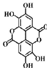
Ellagic Acid (EA)
